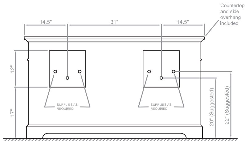
REAR
